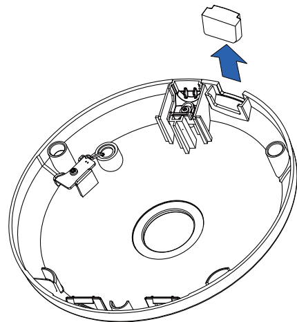
Slide cover
